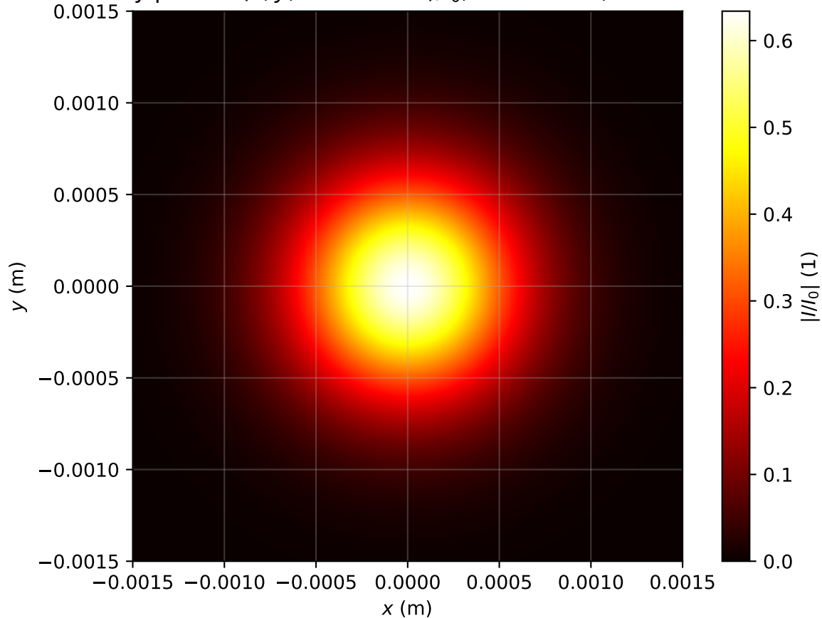
Intensity profile I(x, y, z = 2.070m)/I_0 , \text{Pin}=0.3\text{Pcr} , artificial time
